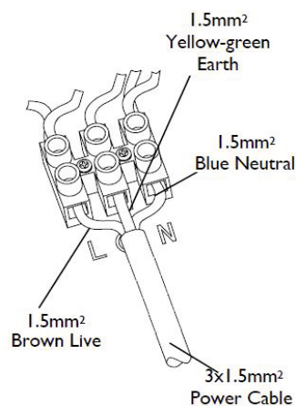
Fig.4 connect the wire
